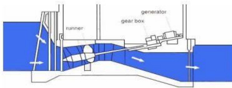
Tubular turbines
