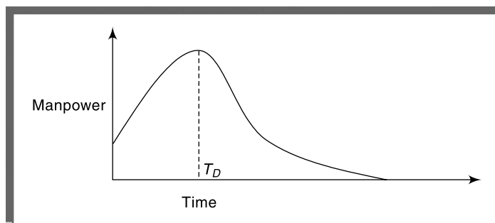
FIGURE 5.3 Rayleigh–Norden Curve
